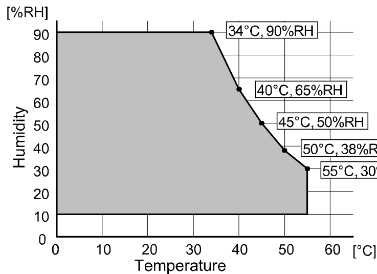
Figure 22-1 Operating Temperature and Humidity Range (Printing)
